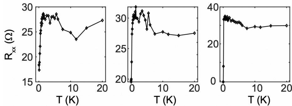
Zhou et al, arXiv:2106.07640 ( non-twisted rhombohedral tri-layer graphene)
